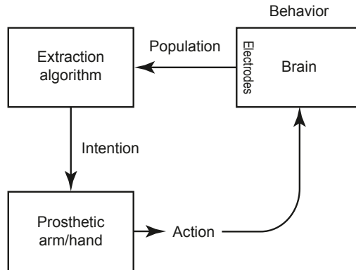
Figure 20.2 Neural prosthetic scheme: Electrodes in the brain record single-unit activity. Many units are recorded simultaneously and this population is processed with an extraction algorithm. This algorithm is a model of the transformation between neural activity and movement intention. The model generates an estimate of the intended movement signal, and this serves as the control signal for an external device (here, a prosthetic replica of the arm and hand). The prosthetic device moves according to the estimated intention signal, and its action is visualized by the subject who registers any errors in the desired movement. The error drives a learning process in the brain which modifies the neural output to reduce the error signal. Essentially, the brain is learning the extraction algorithm. This closed loop induces powerful learning, leading to high prosthetic performance.
